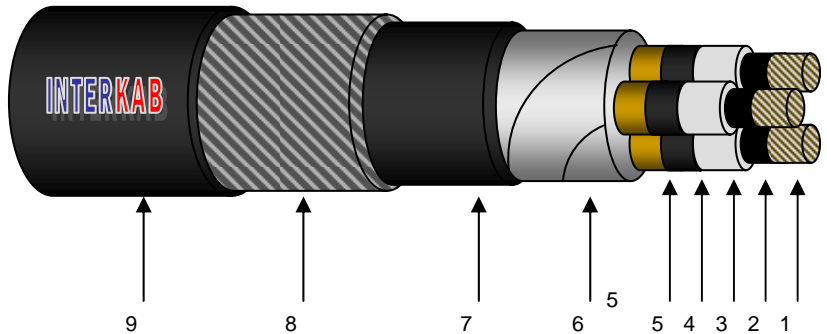
Multi Core Armoured Cables
